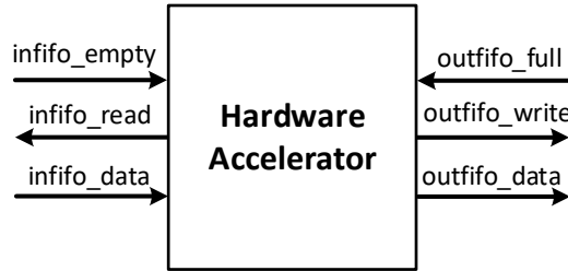
Figure 2: Hardware accelerator interface.
