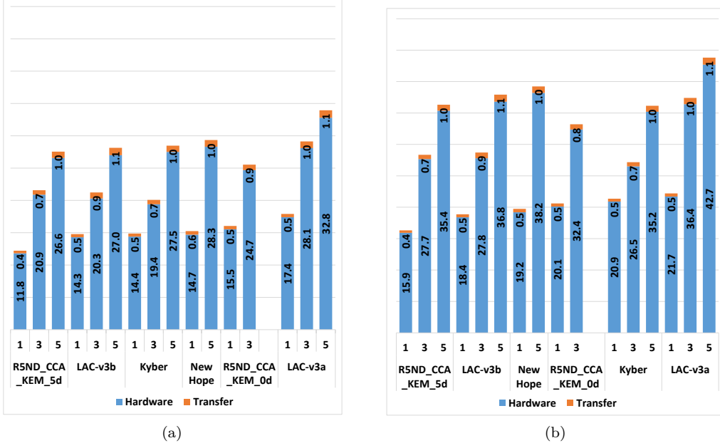
Figure 6: Execution Time for (a) Encapsulation and (b) Decapsulation ( \mu s ) on Artix-7
