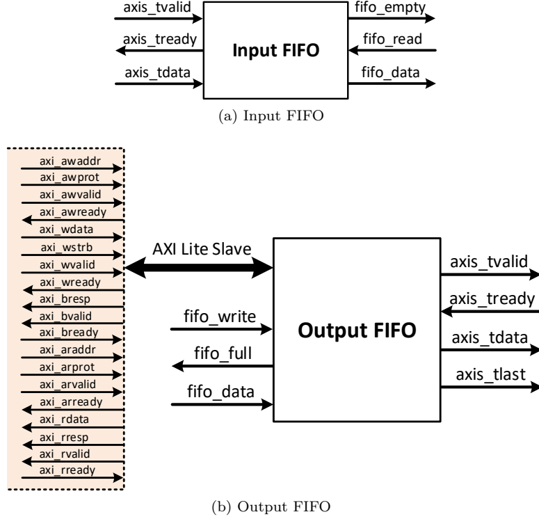
Figure 3: The Input and Output FIFO Interface.
