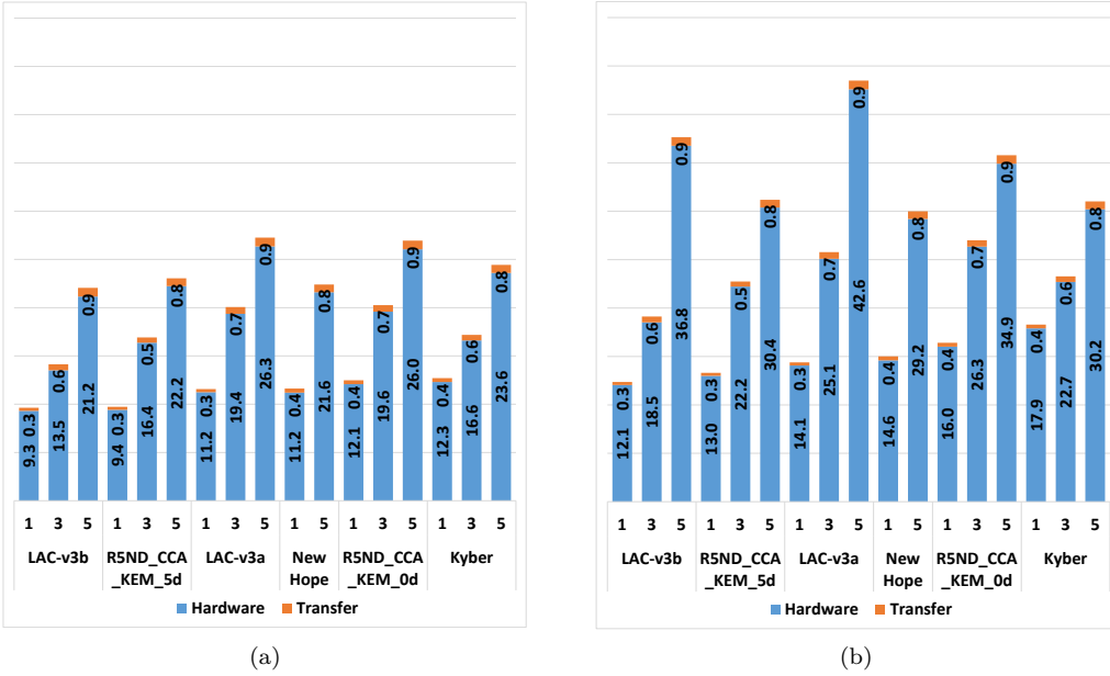
Figure 7: Execution Time for (a) Encapsulation and (b) Decapsulation ( \mu s ) on Virtex7
